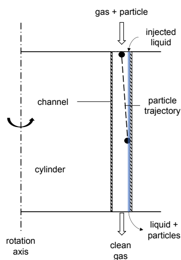
Figure 14. Liquid flushing in a vertical RPS.
