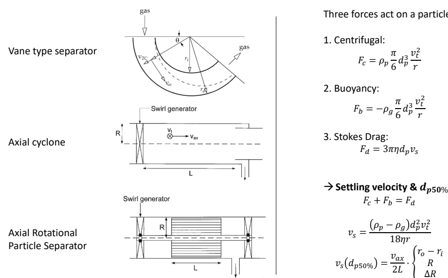
Figure 10. Centrifugal separation methods.
