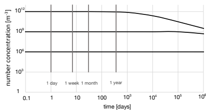
Figure 5. Particle number concentration versus time for simple monodisperse coagulation.
