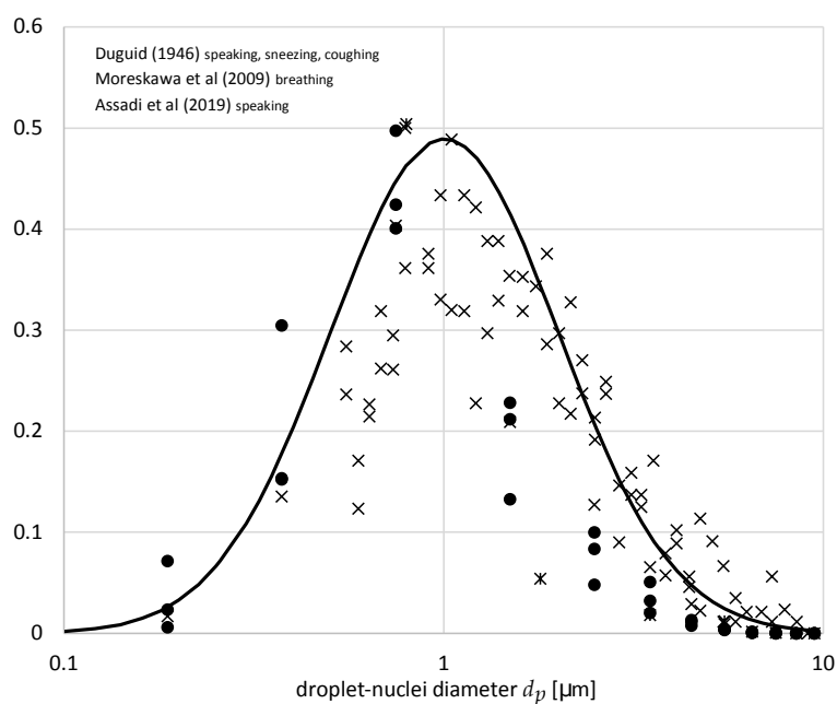
Figure 4. Probability density function of the droplet nuclei emitted by humans.
